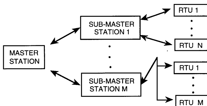
Figure A.9 —Single master station, multiple sub-master stations, multiple RTU(s)
